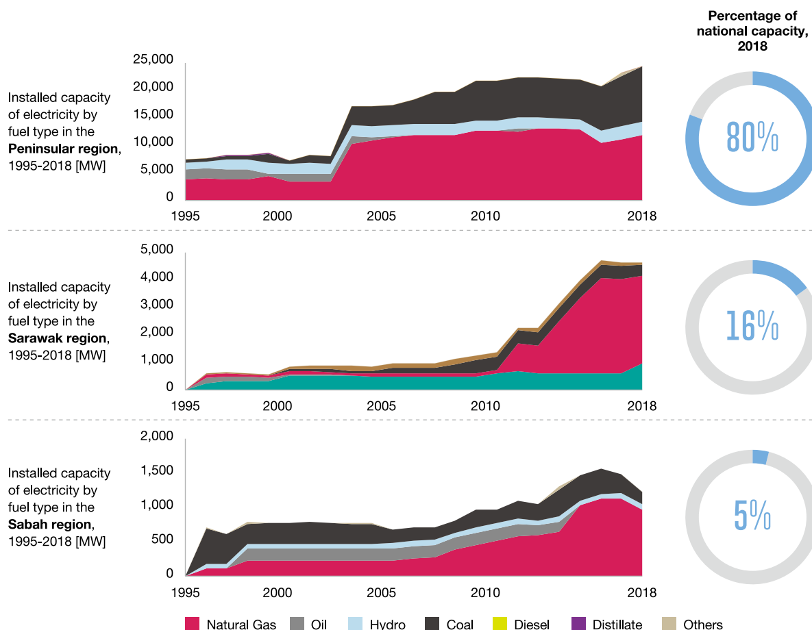
Figure 3-3: On-grid installed capacity by region, 1995-2018
