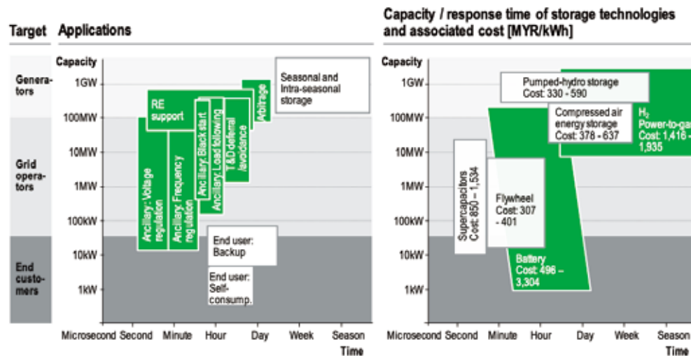
Figure 6-14: Energy storage applications and technologies
