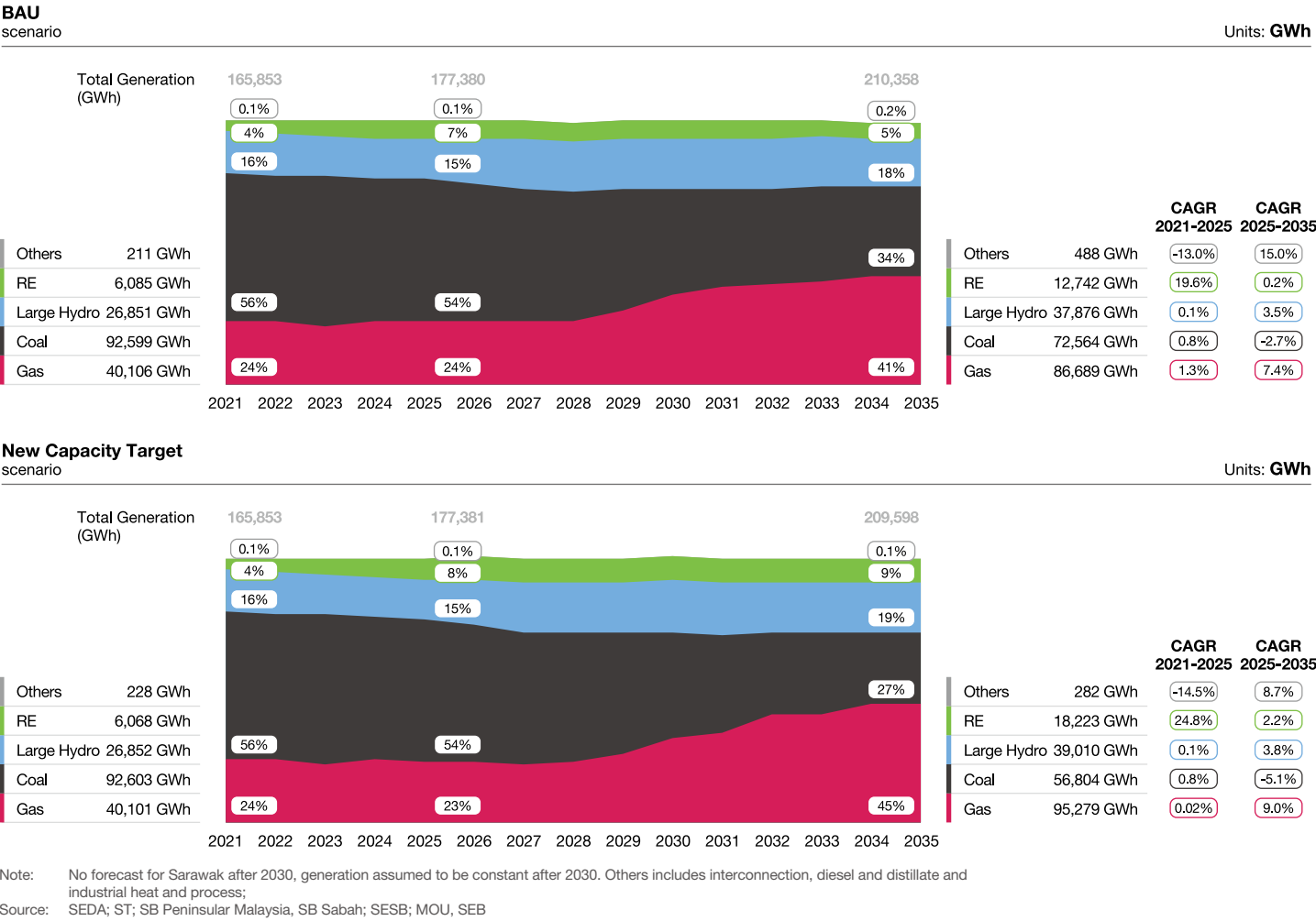
Figure 7-13: Generation mix for Malaysia for BAU and New Capacity Target scenarios, 2021-2035
