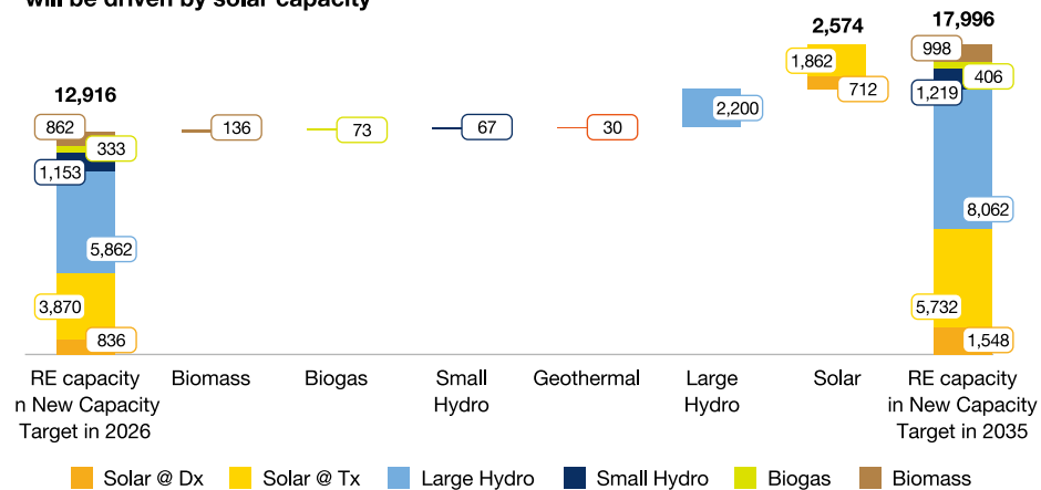
Figure 5-10: Breakdown of additions for RE capacity for Malaysia post 2025 – New Capacity Target scenario
